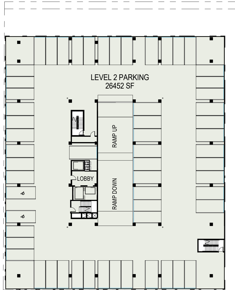
LEVEL 2 FLOOR AREA (RETAIL PARKING LEVEL 2)
